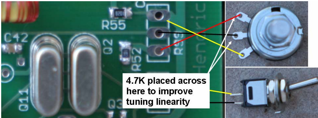
Figure 91. Tx VXO tuning linearity improved by using an external 4.7K resistor
