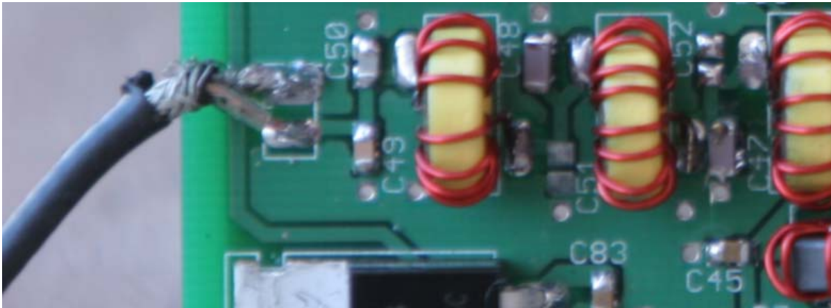
Figure 69. Antenna coax connection to transceiver. Upper connection is ground, lower is antenna.
