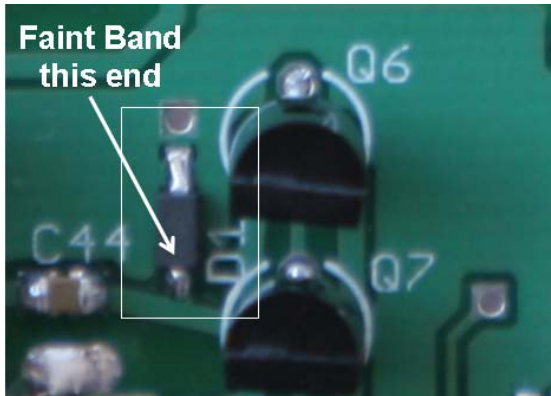
Figure 67. Close up of Zener diode D1 with band orientation
