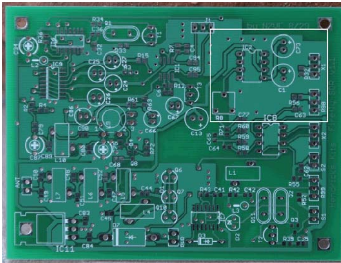
Figure 25. Top side parts location of the CW side tone monitor amplifier
