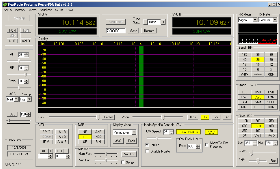
Figure 87. Generic settings – NB on, 500 Hz filter, CWU, proper band selected (30m here)
