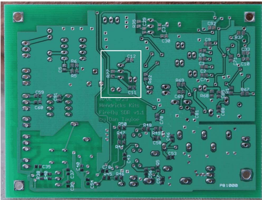
Figure 19. Bottom side parts location of 6v regulated
