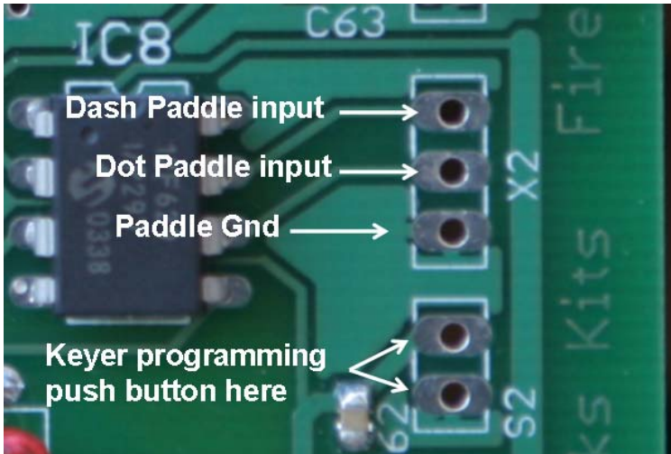
Figure 74. Connections for keyer paddle inputs (X2) and for keyer programming push button switch (S2)
