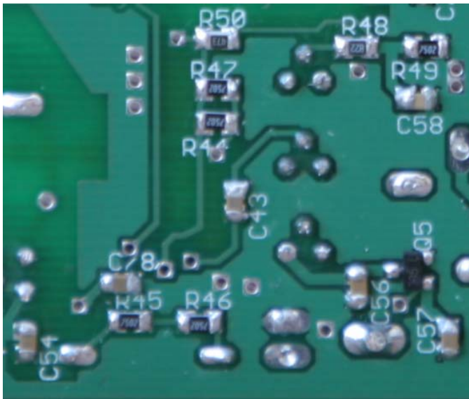
Figure 60. Bottom side TX buffer with parts installed
