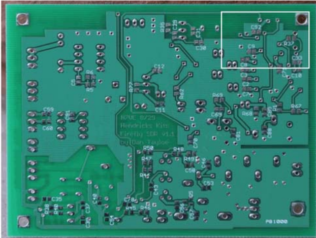
Figure 39. Bottom side location of the receiver crystal oscillator circuitry
