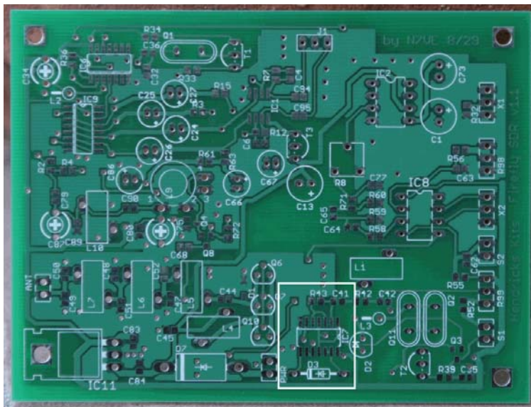
Figure 57. Top side location of the TX Buffer circuit
