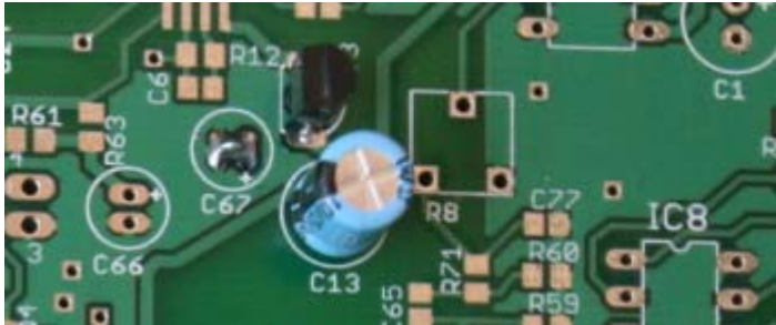
Figure 22. 6v regulator with C67 shorted and C13 installed. Note T3 flat side orientation and C13 stripe orientation.
