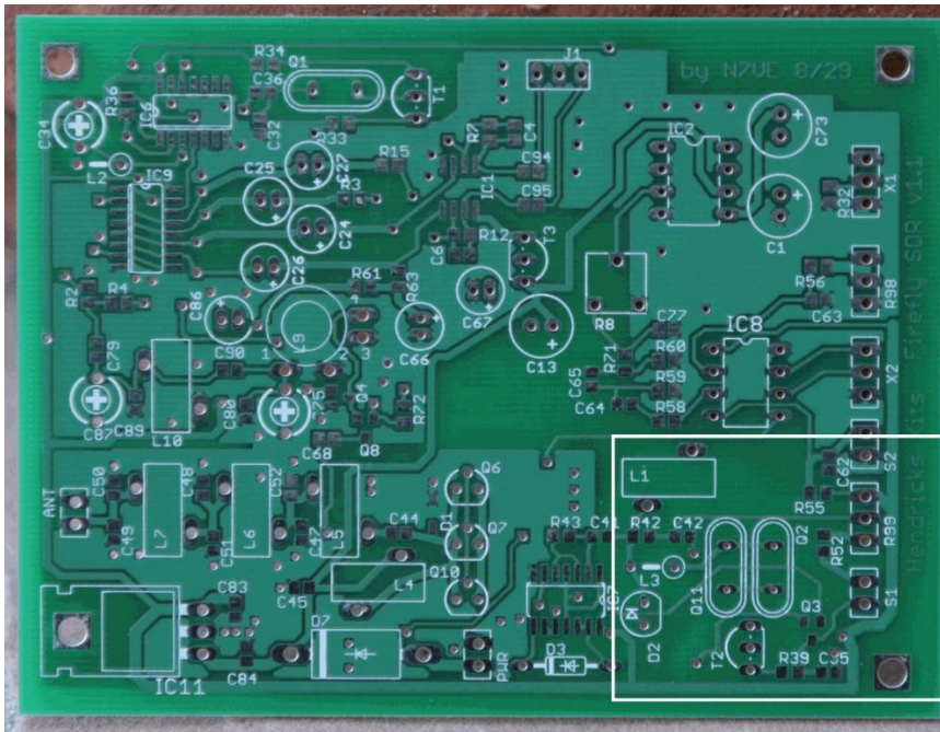
Figure 53. Top side location of the transmitter VXO
