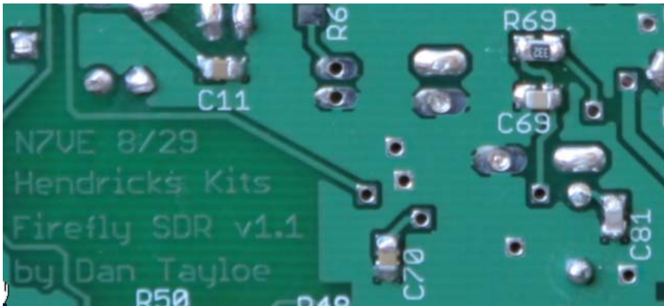
Figure 50. Close up of bottom T/R parts. R69, C69, C70 and C81
