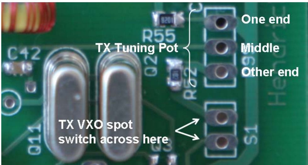
Figure 76. Connections for TX spot switch (S1) and TX VXO 10K tuning pot (R99).
