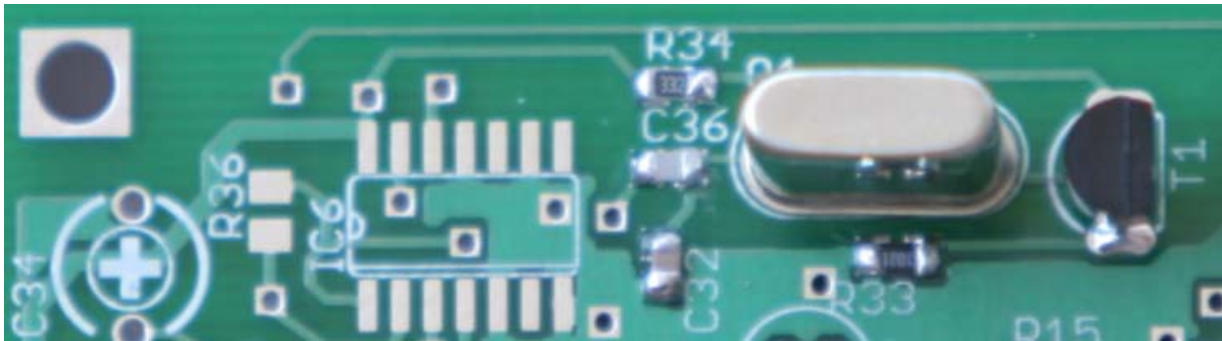
Figure 36. Top side receiver LO parts mounted
