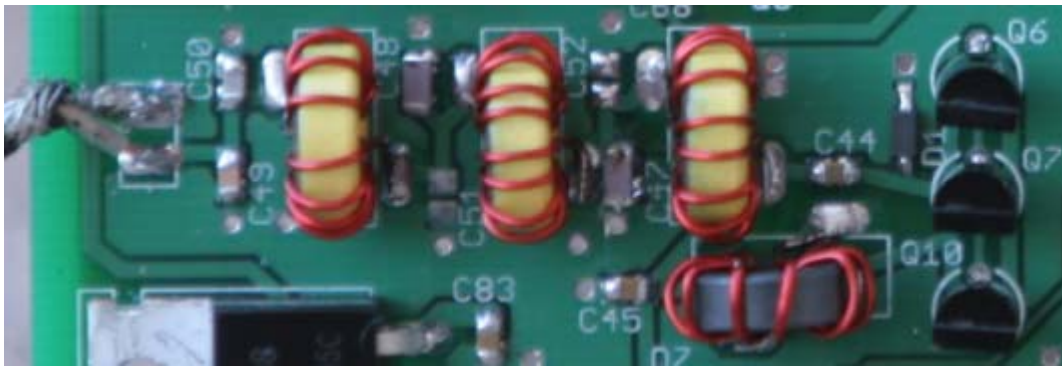
Figure 65. Top side parts view of the PA circuit. C50 (left top end cap) not used on the 30m version.
