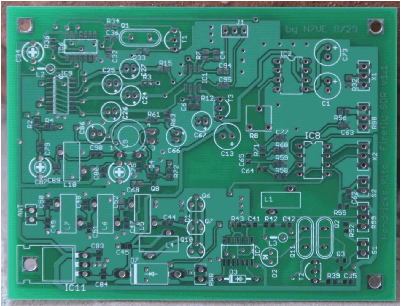
Figure 16. Top side view of the Firefly SDR PC board
