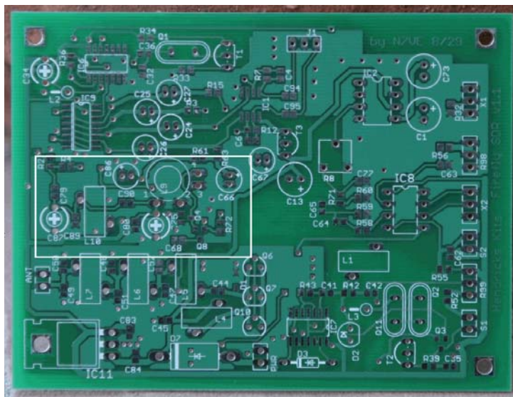
Figure 48. Top placement of receiver front end and T/R switch
