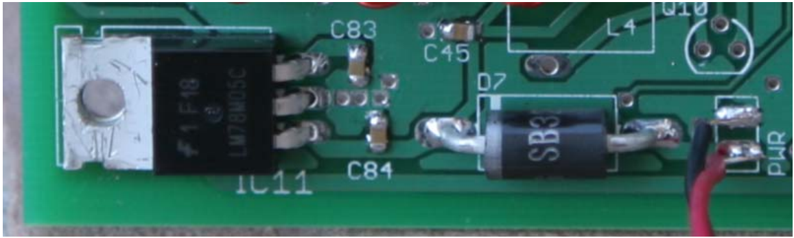
Figure 20. Top side view of 5v regulator, protection diode, and 9v temporary connection. Note D7 diode polarization!
