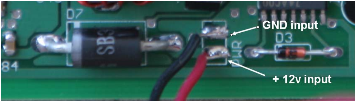
Figure 78. Connections for 12v to the board
