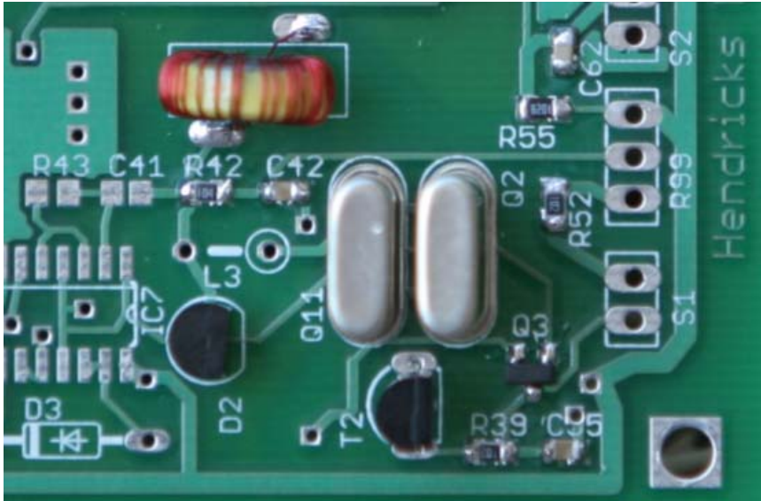
Figure 55. Close up of top side installed transmitter VXO parts
