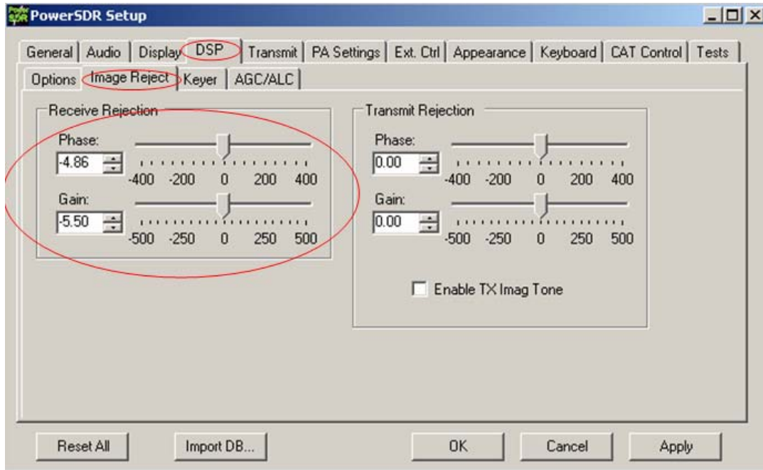
Figure 86. DSP/Image Reject tab used to null opposite sideband signal
