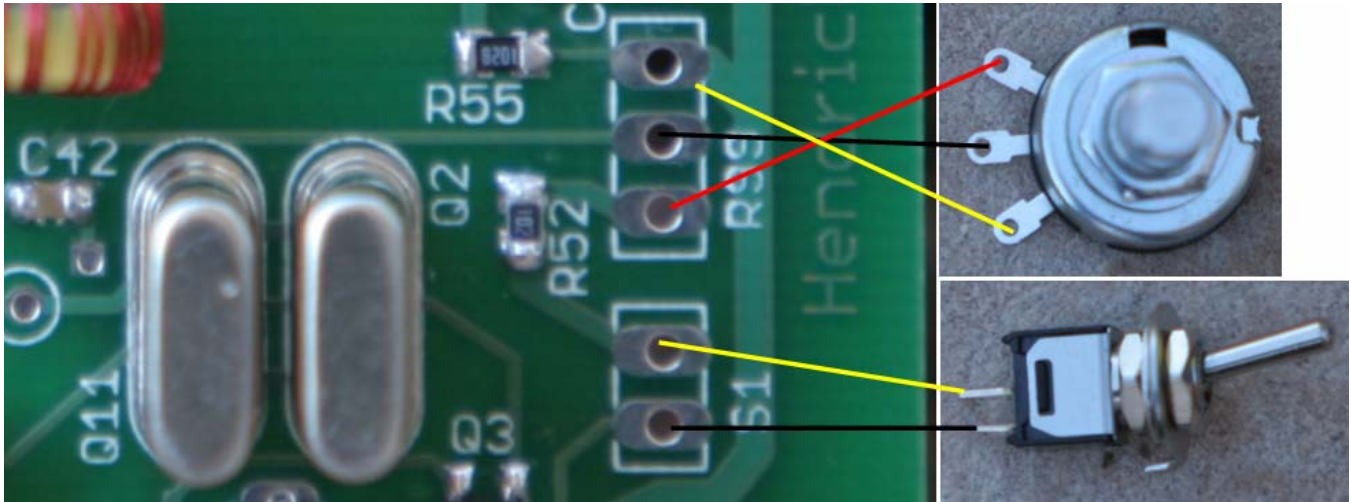
Figure 77. Visualization of TX tuning pot and VXO spot switch connections. Switch shown “Spot On”.
