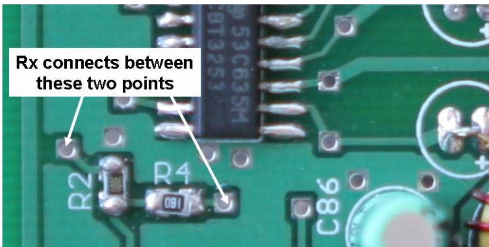
Figure 90. If the input attenuator is increased, Rx can be placed across the above 2 points, keeping R1 as is.
