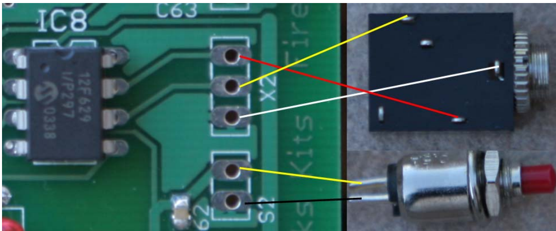
Figure 75. Visualization of paddle jack and keyer programming switch connections
