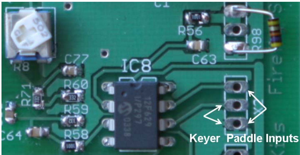
Figure 62. Location of keyer paddle inputs to test the T/R switch
