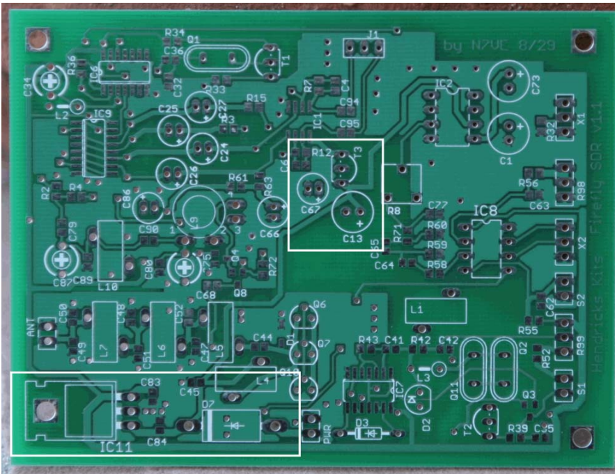
Figure 18. 5v, 6v Regulator and 12v input areas highlighted, top side
