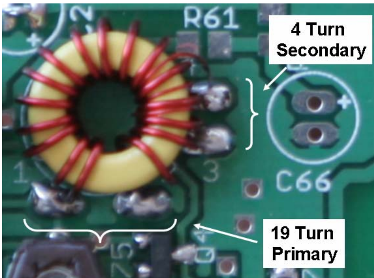
Figure 52. Close up of input receiver filter inductor L9. 30m values shown. For other bands see text.
