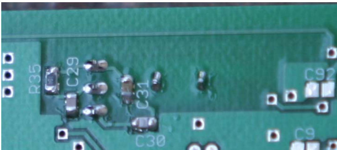
Figure 37. Bottom side receiver LO parts mounted
