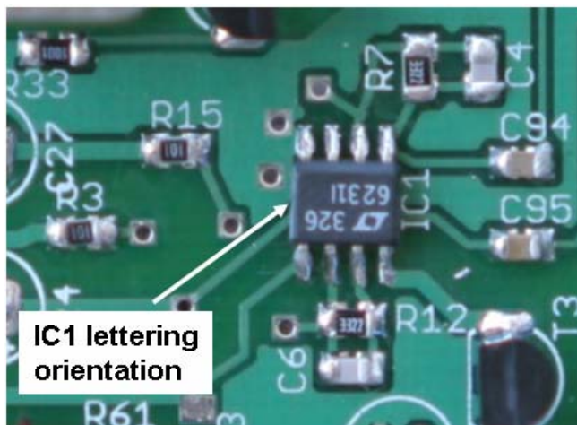
Figure 47. Close up of the parts in the audio preamp stage (top side only)
