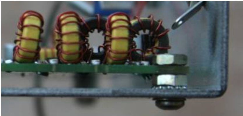
Figure 82. Mount all four corners of the main board using the mounting hardware as shown.
