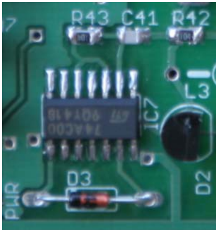
Figure 59. Top side TX buffer parts installed. IC7, D3, R43, C41
