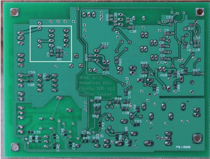
Figure 26. Bottom side parts location of the CW side tone monitor amplifier
