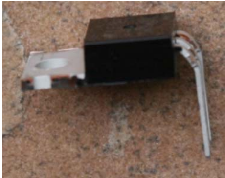
Figure 21. Lead forming of the LM78M05 5v regulator before installation
