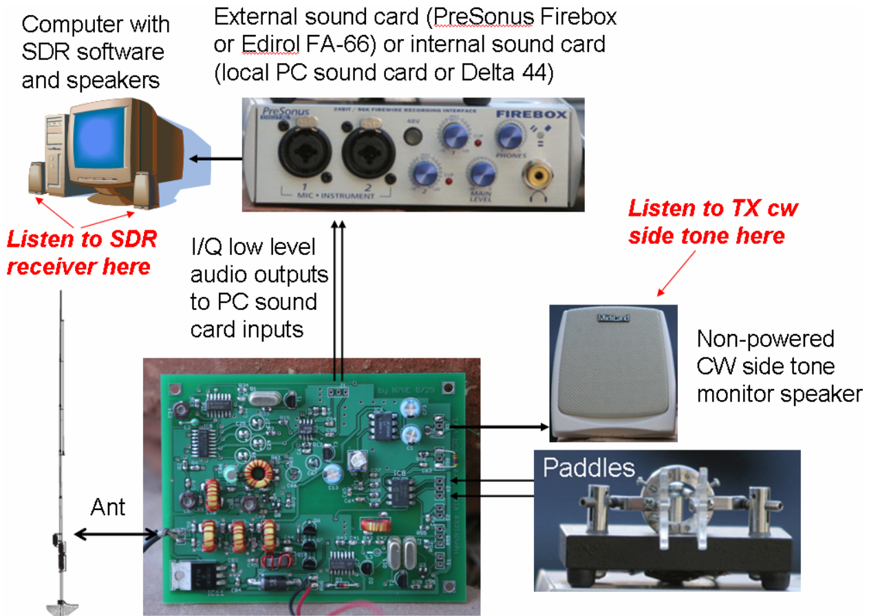
Figure 81. Diagram of the major external interfaces of the Firefly SDR, less front panel controls.
