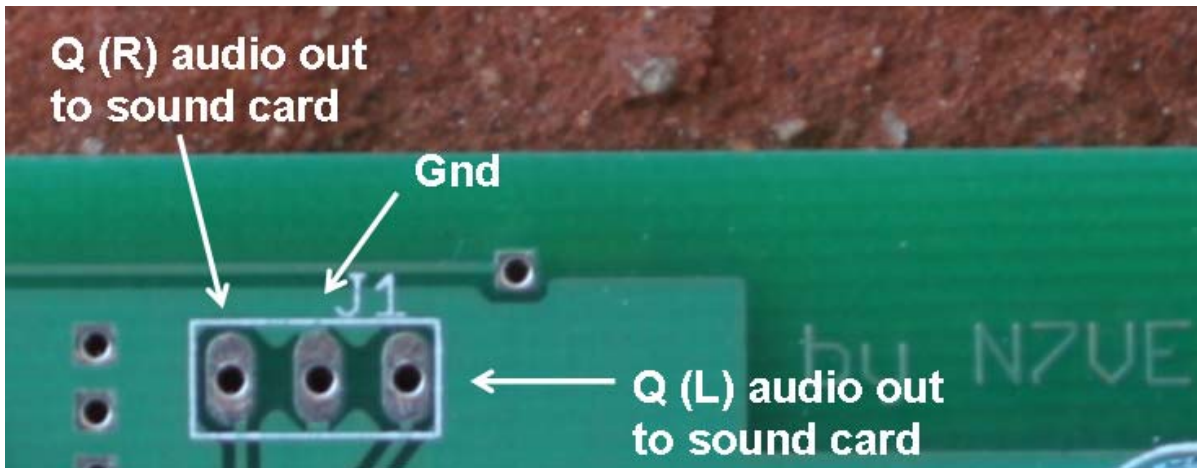
Figure 70. Connections for J1, I/Q (R/L) audio output to the PC sound card input
