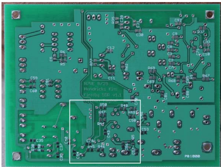
Figure 58. Bottom side location of the TX buffer circuit.
