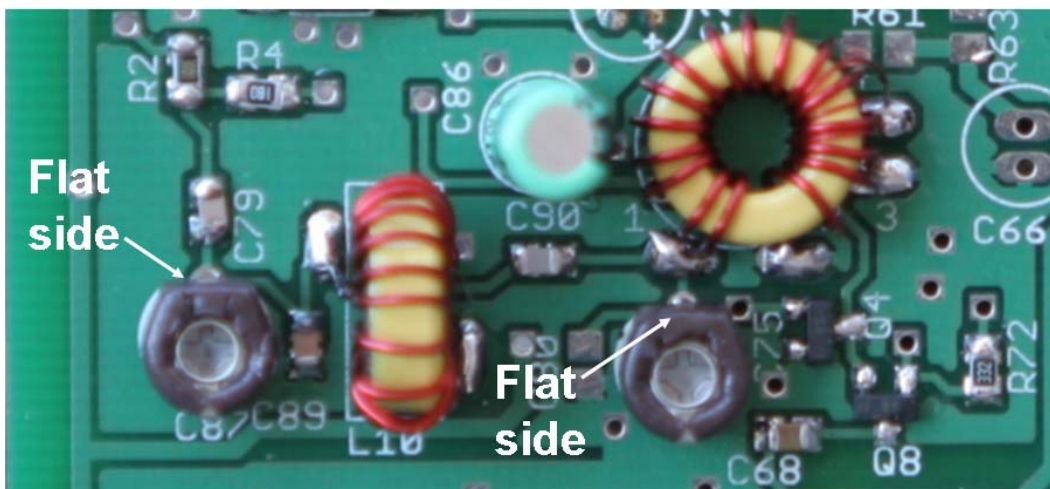
Figure 51. Close up of top side receiver front end and T/R switch
