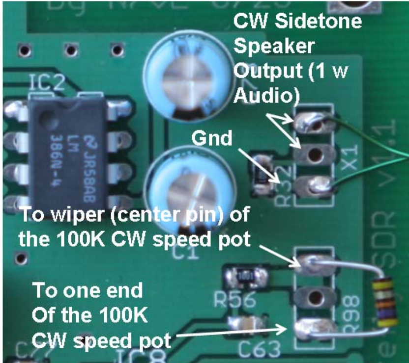
Figure 72. Connections for X1 and R98, CW side tone monitor speaker and 100K CW speed pot.
