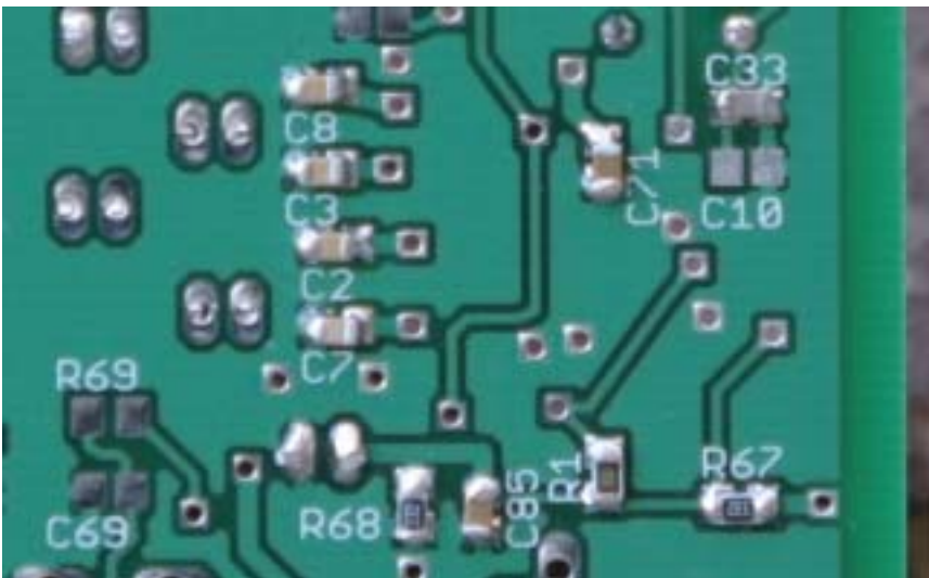
Figure 45. Close up of bottom side detector circuit
