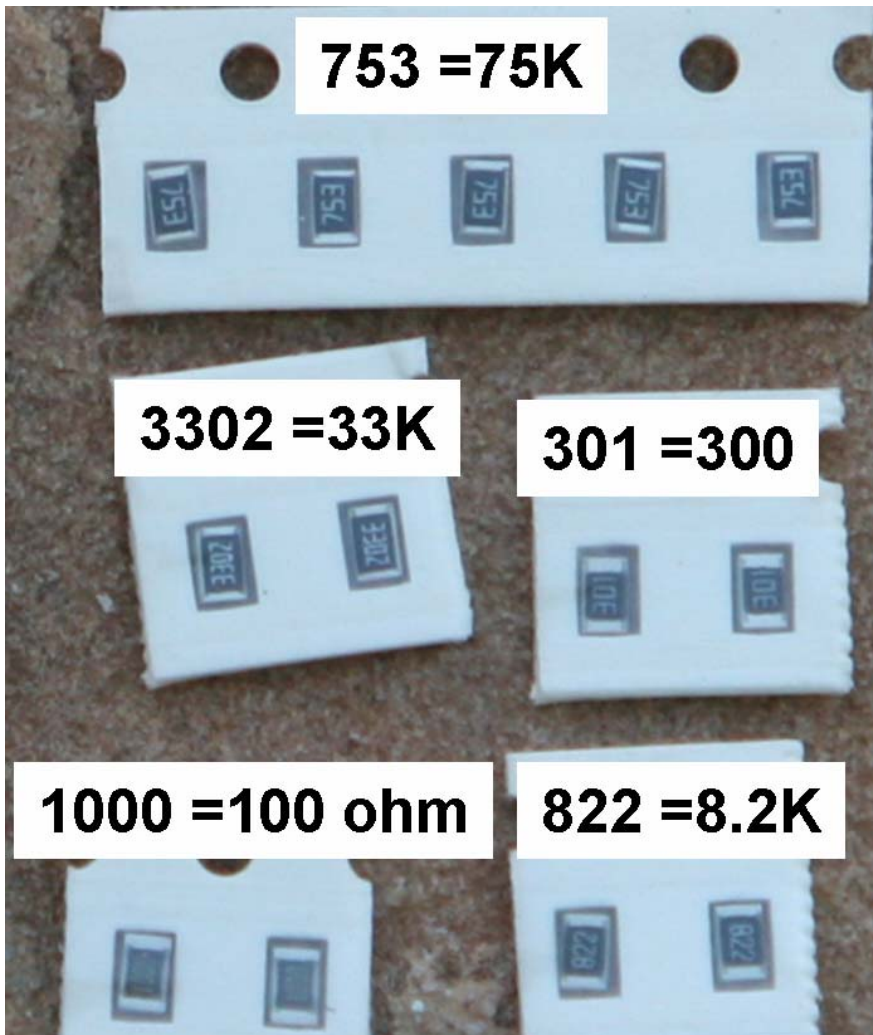
Figure 15. The remainder of the surface mount resistors.
