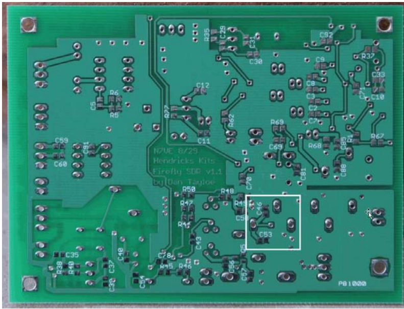
Figure 64. Bottom side view of the PA circuit
