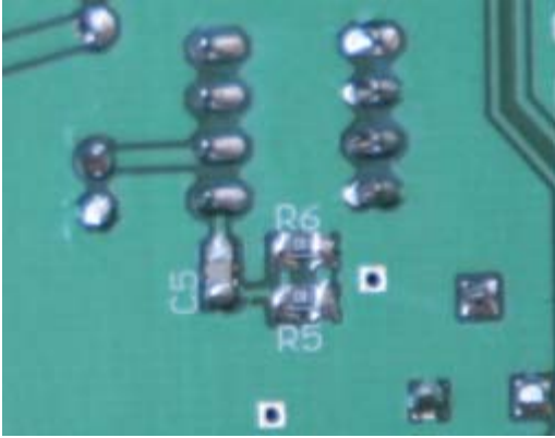
Figure 28. Bottom side installation of R5, R6, and C5.
