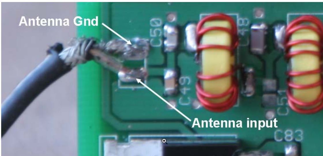
Figure 79. Antenna Connections
