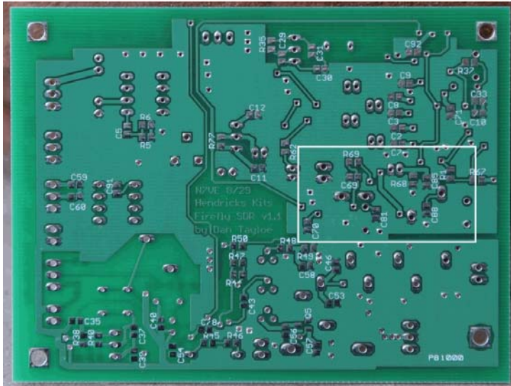
Figure 49. Bottom placement of receiver front end and T/R switch
