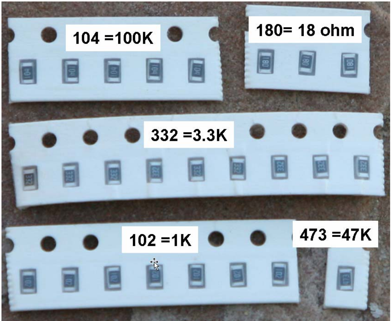
Figure 14. Close up of part of the surface mounted resistors
