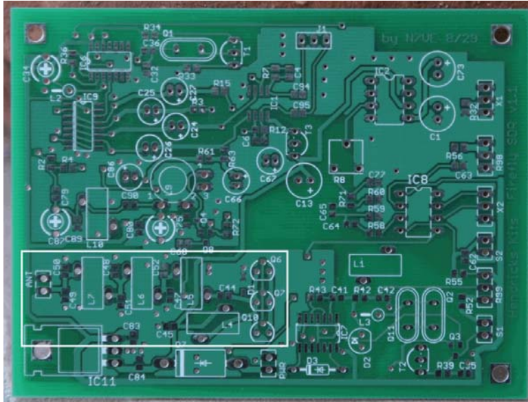
Figure 63. Top side view of the PA circuit
