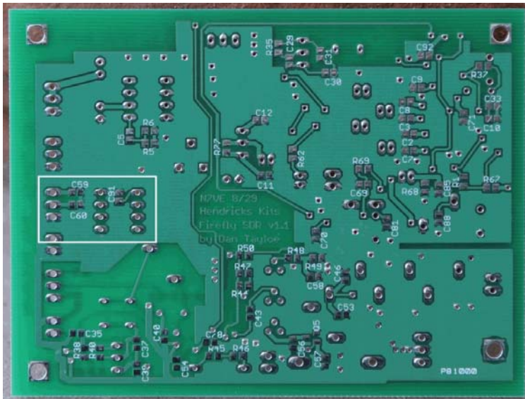
Figure 30. Bottom side location of keyer chip components C59, C60, and C91
