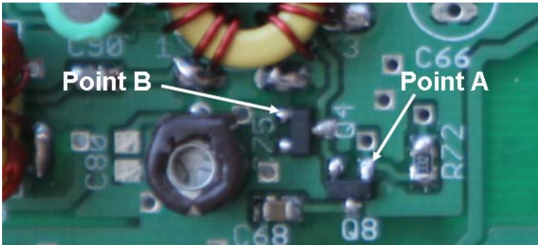
Figure 61. Top side test points for the T/R switch in the receiver front end
