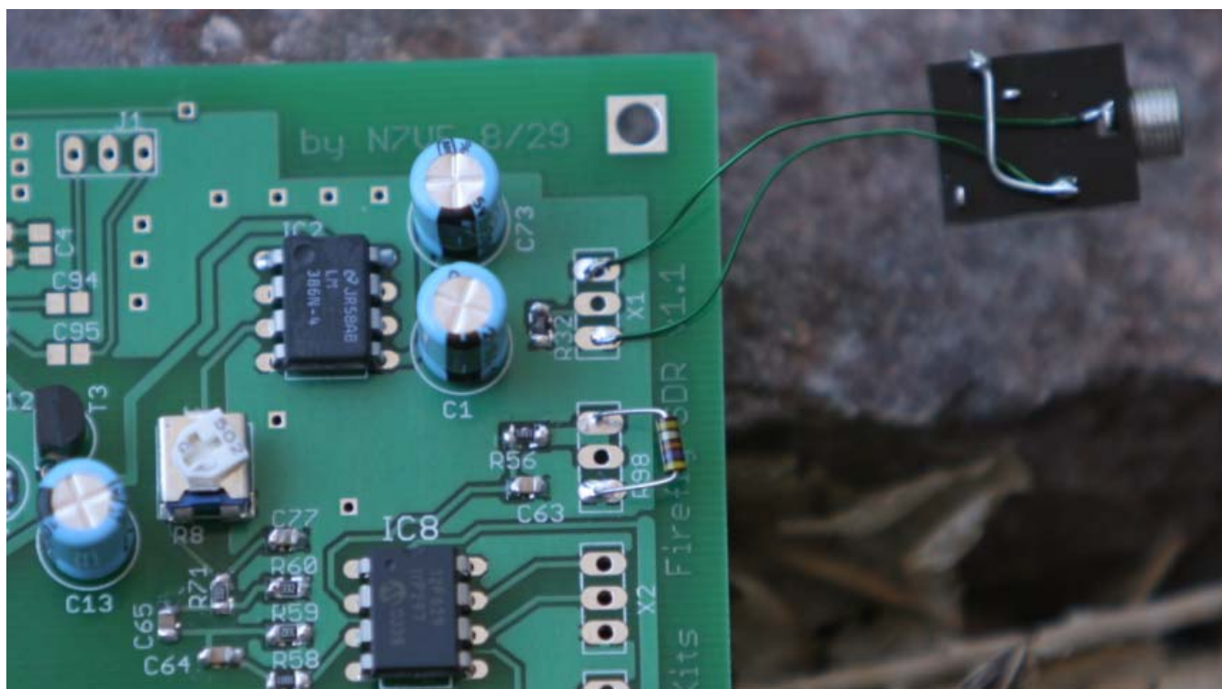
Figure 33. Temporary connection of a headphone jack to test the CW side tone monitor speaker output
