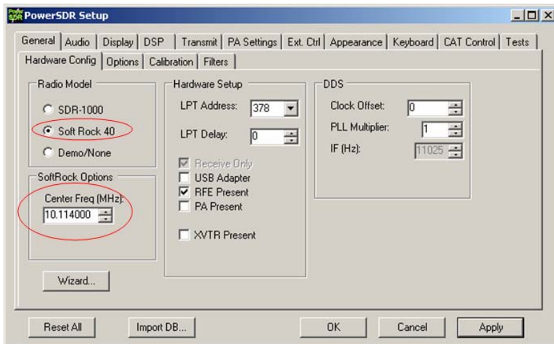
Figure 84. Select the setup tab to get to this window. Select SoftRock, and set the center frequency.
