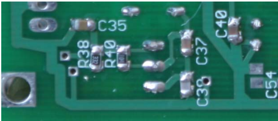
Figure 56. Close up of the bottom side installed transmitter VXO parts
