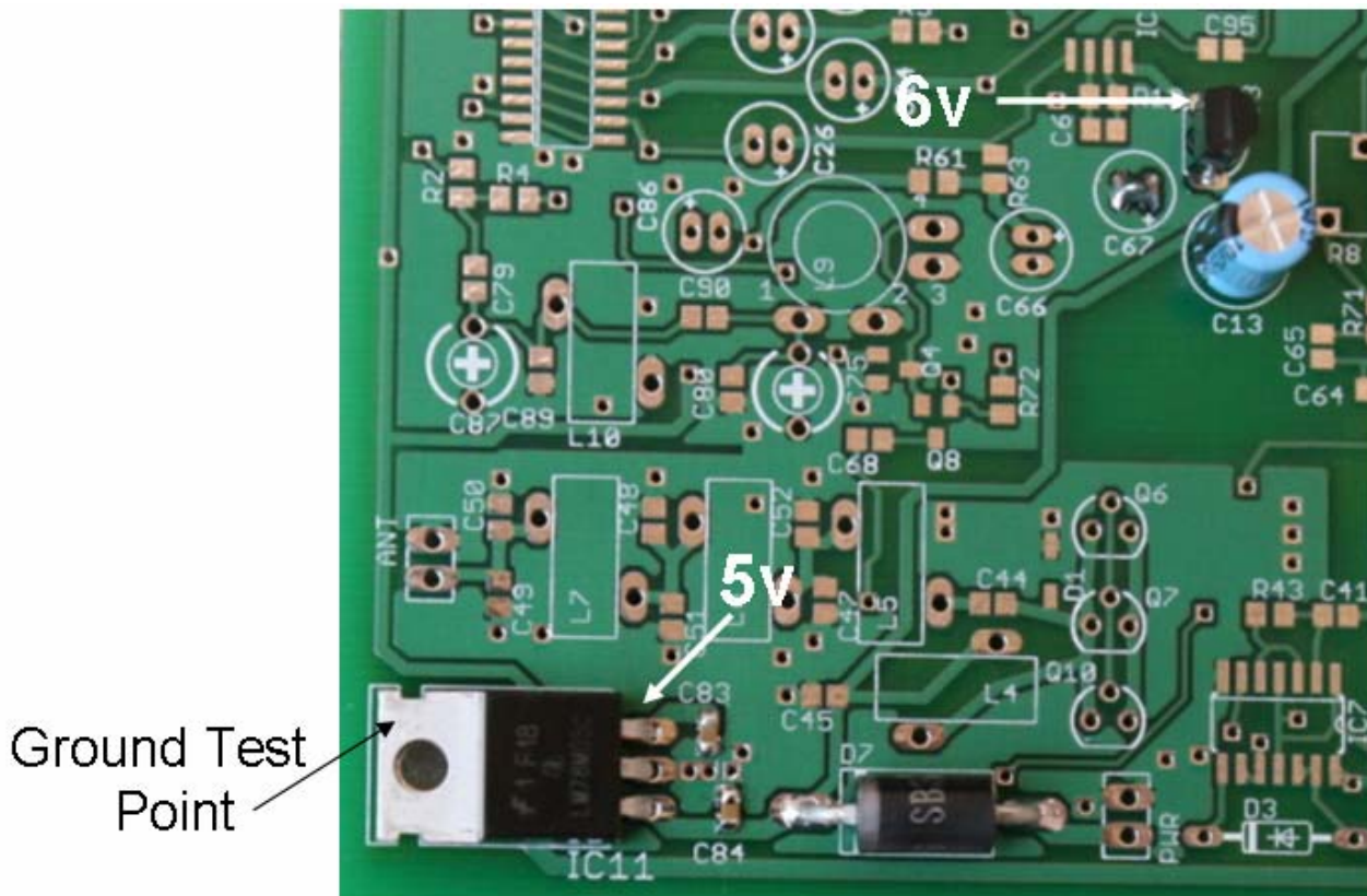
Figure 24. Ground point and 5v/6v regulator output test points
