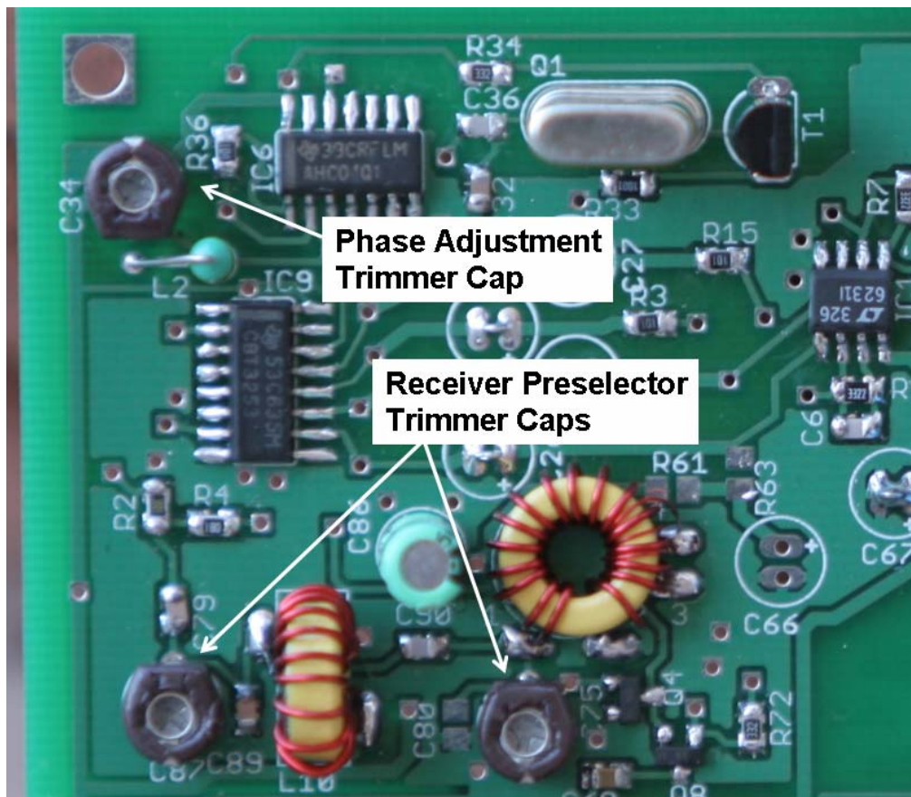
Figure 88. Adjustment points for tuning up the receiver.
