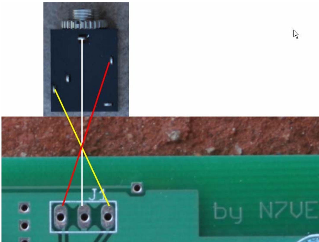
Figure 71. Connections of the I/Q audio output to its audio jack
