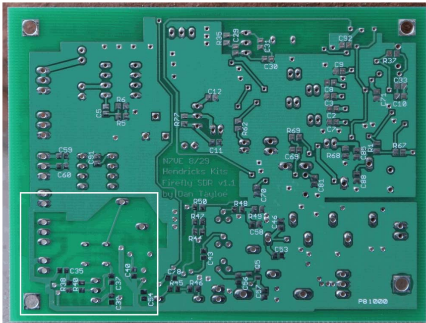
Figure 54. Bottom side location of the transmitter VXO
