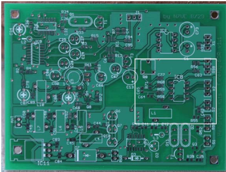
Figure 29. Top side location keyer circuitry
