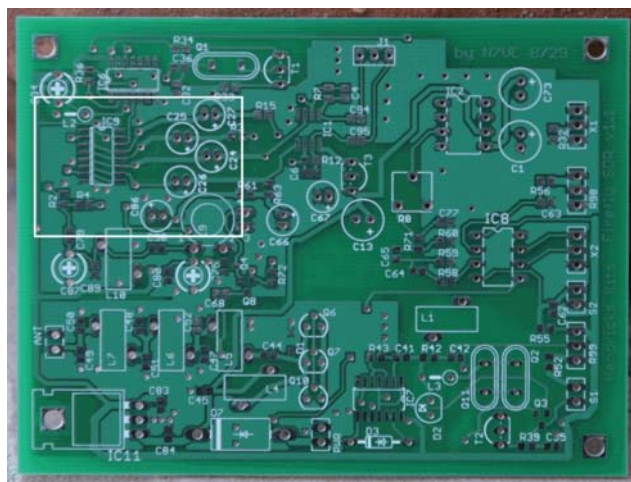
Figure 42. Top side location of the detector circuit
