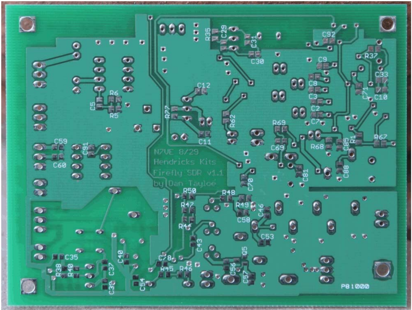
Figure 17. Bottom side view of the Firefly SDR circuit board.
