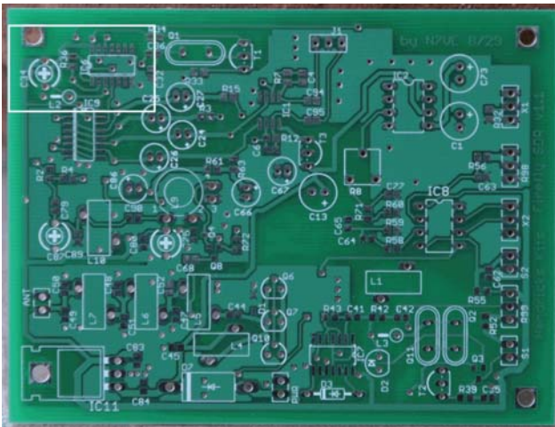
Figure 38. Top side location of the receiver crystal oscillator circuitry
