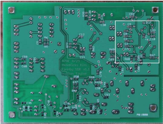
Figure 43. Bottom side location of the detector circuit
