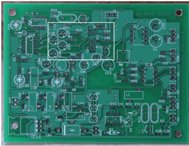
Figure 46. Top placement of receiver audio preamp stage
