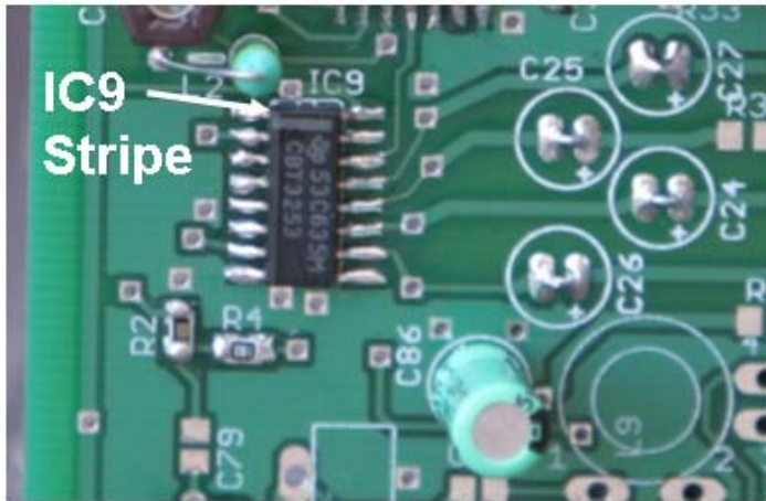
Figure 44. Top side Detector, R2, R4, C86, and IC9
