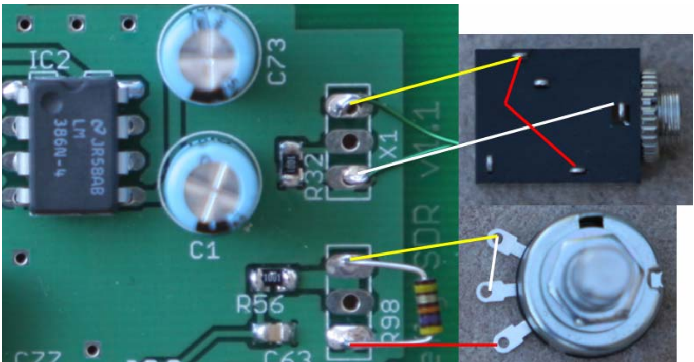
Figure 73. Connections to CW mon speaker jack, CW speed pot. Remove temporary resistor across R98.
